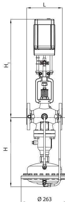
AME 55, 56 + AFQM 6 (DN 40, 50)
