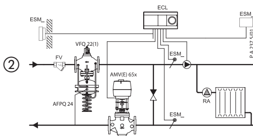
Direct-connected heating system
