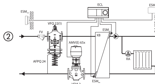
Indirectly connected heating system
