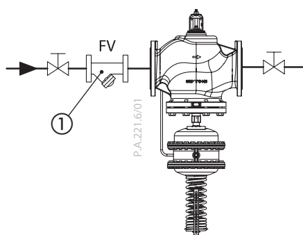
Direct-connected heating system
