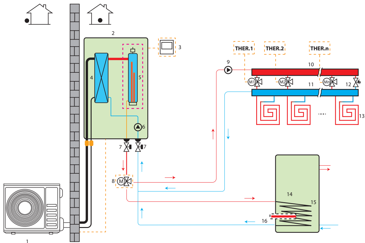
Figure 2.1.1: Space heating
