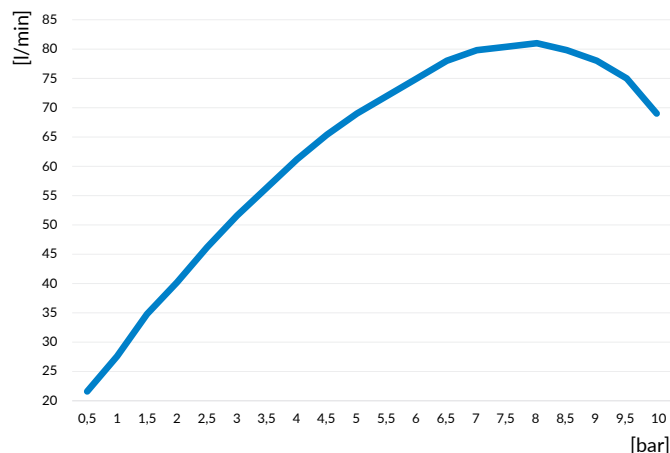
Fig. 7. Venting performance characteristics
