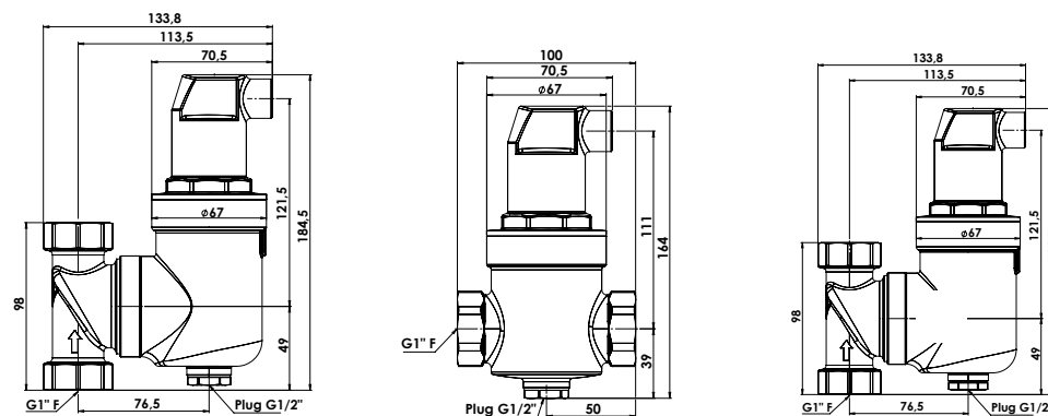
Fig. 2. Dimensions of air separators (respectively from left) AAS 260 / 280 / 281
