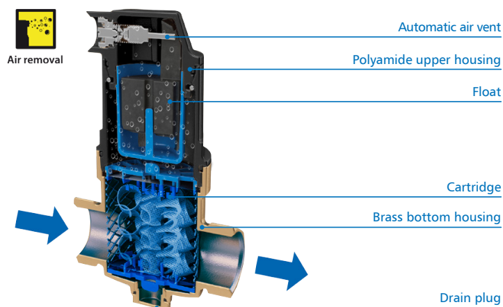
Fig. 1. Construction of the AAS air separator
